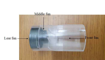
Figure 2. Flow calculation turbine of 'The Spirokit'
